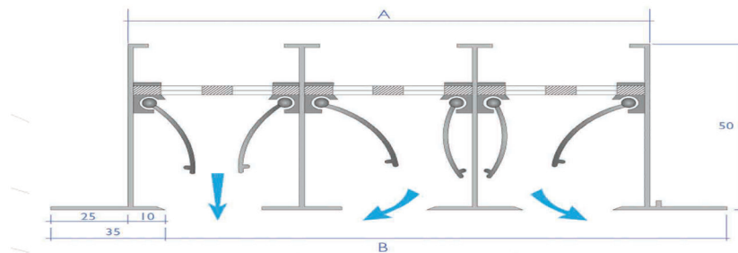
Type SLSD-P with Deflectors and Hit & Miss Dampers
